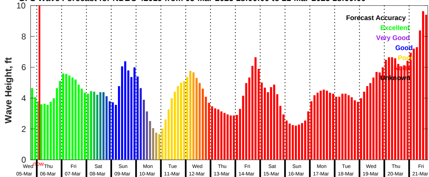
GFS Wave Forecast for NDBC 42019 from 05-Mar-2025 18:00:00 to 21-Mar-2025 18:00:00
