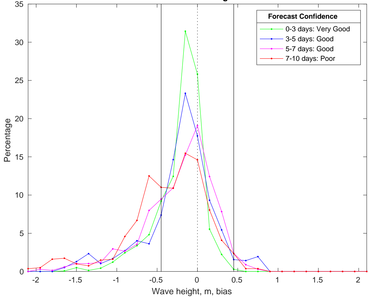
NDBC 42020 vs CMEMS Waves Bias Histogram: 06-Mar-2025
