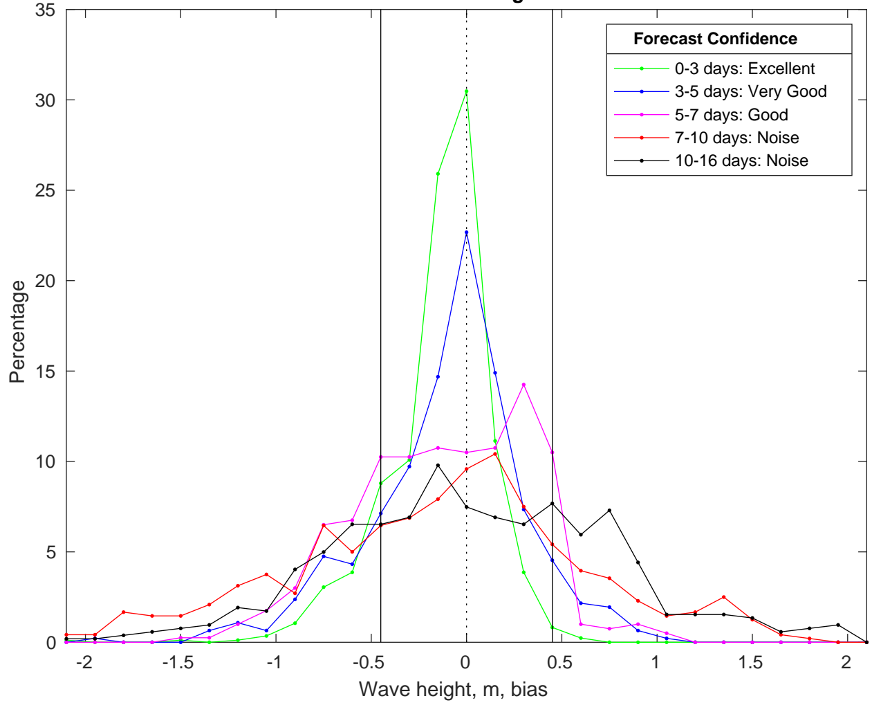
NDBC 42020 vs GFS Waves Bias Histogram: 06-Mar-2025
