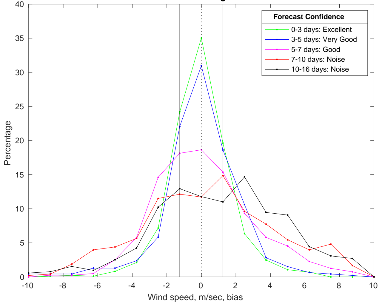
NDBC 42020 vs GFS Winds Bias Histogram: 06-Mar-2025
