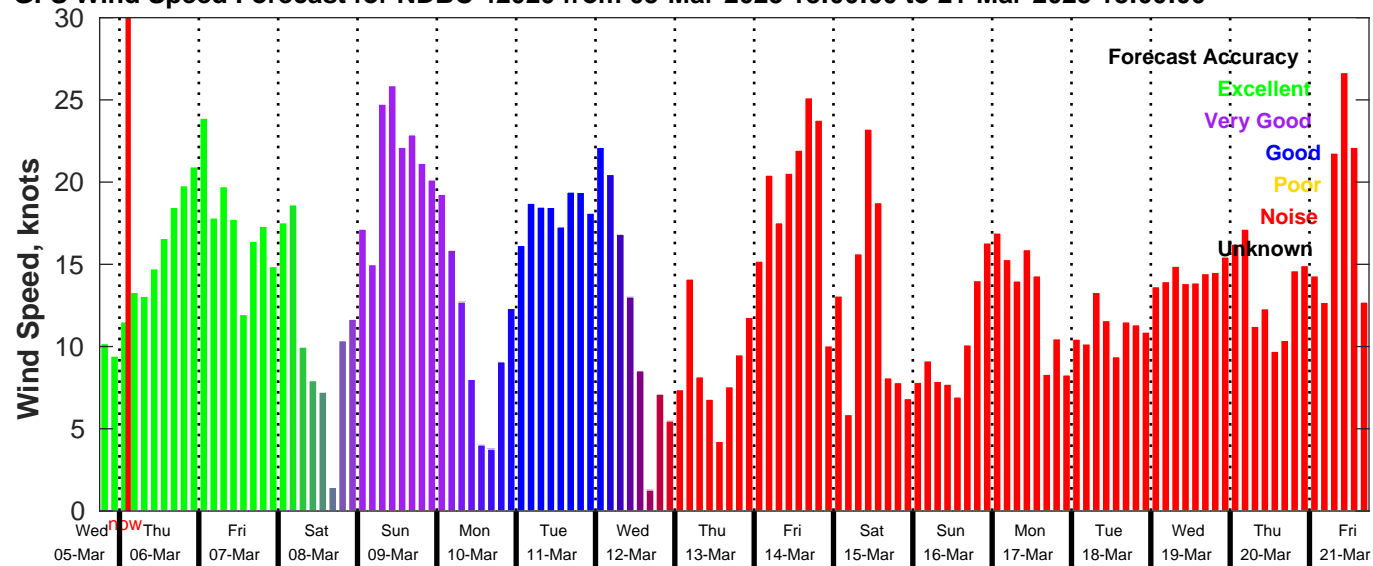
GFS Wind Speed Forecast for NDBC 42020 from 05-Mar-2025 18:00:00 to 21-Mar-2025 18:00:00
