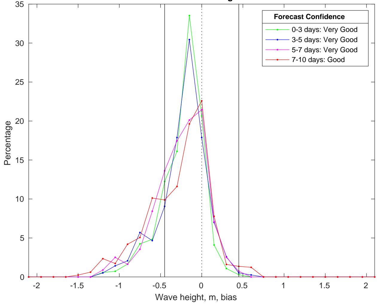
NDBC 42035 vs CMEMS Waves Bias Histogram: 06-Mar-2025
