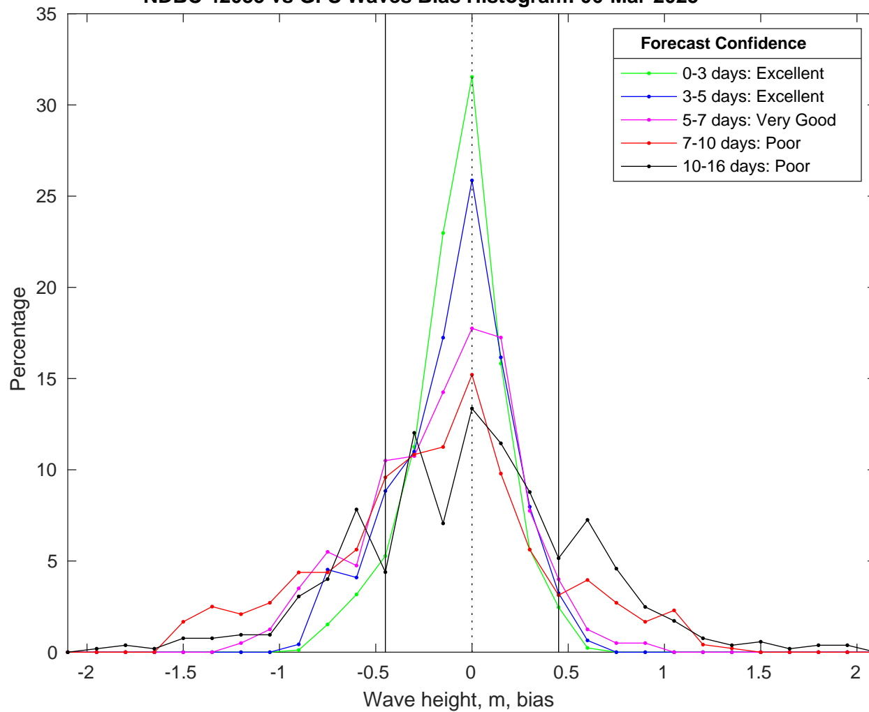
NDBC 42035 vs GFS Waves Bias Histogram: 06-Mar-2025
