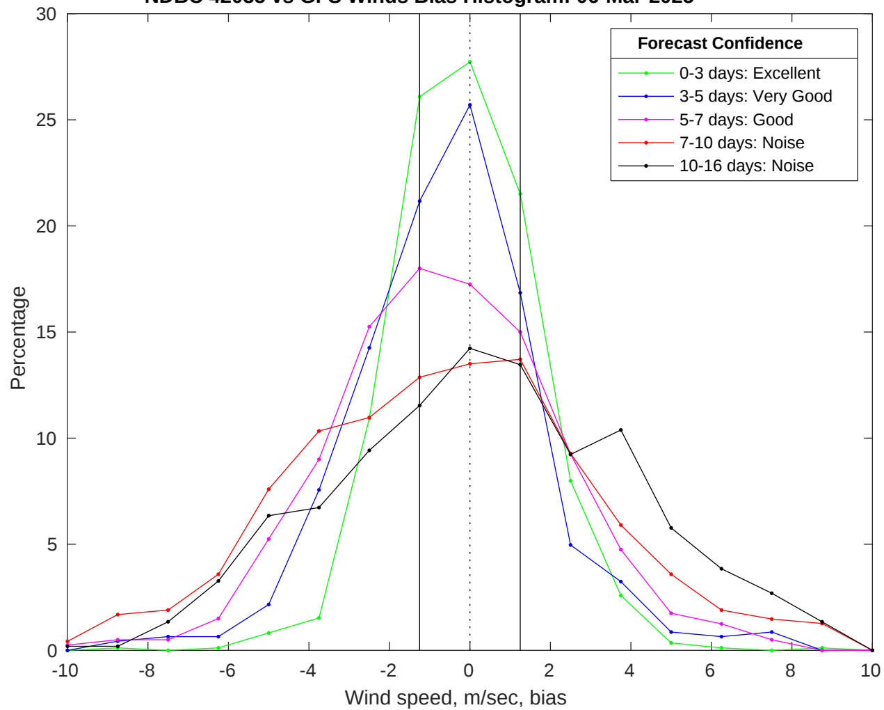
NDBC 42035 vs GFS Winds Bias Histogram: 06-Mar-2025
