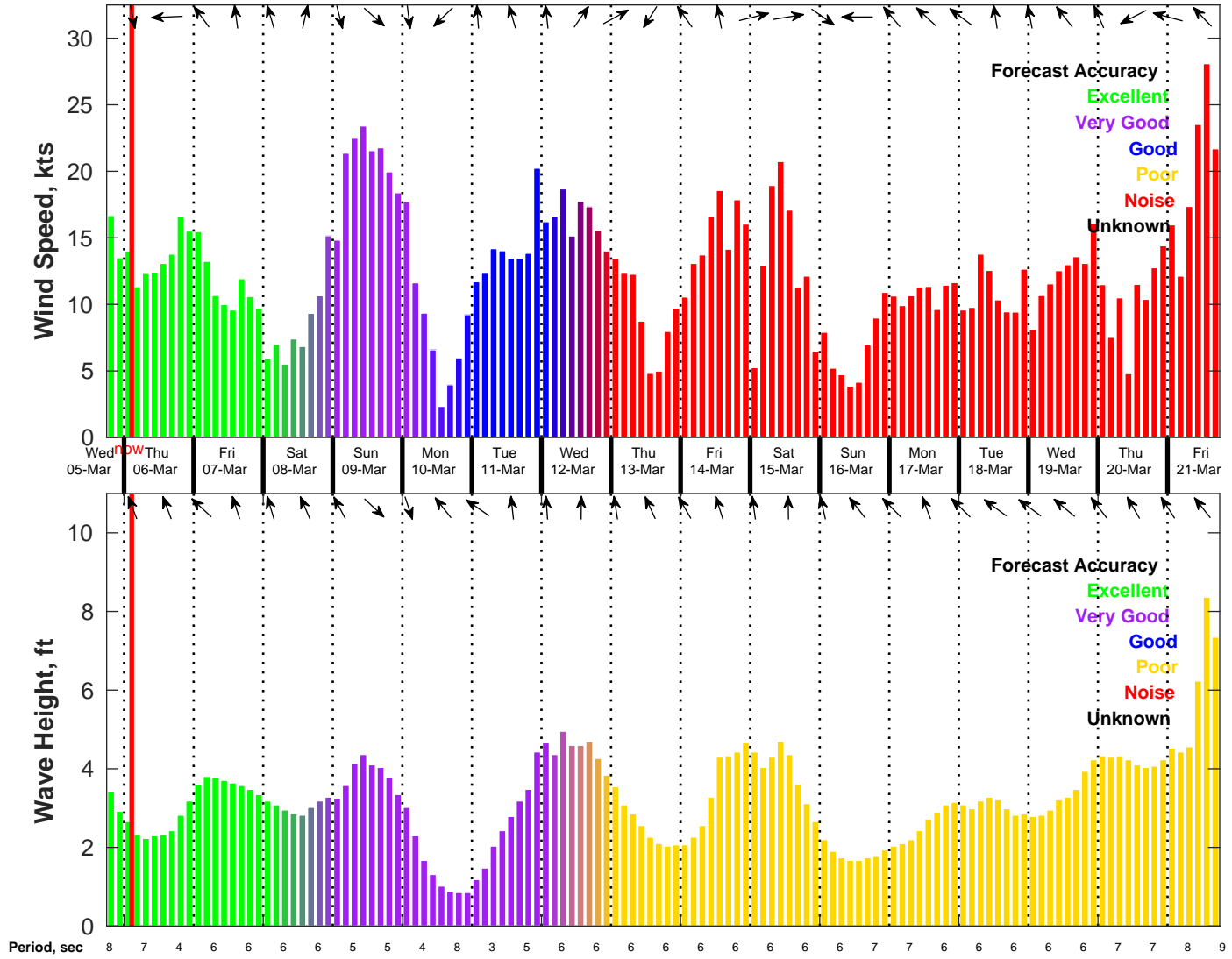
Wind & Wave Forecast for NDBC 42035 from 05-Mar-2025 18:00:00 to 21-Mar-2025 18:00:00
