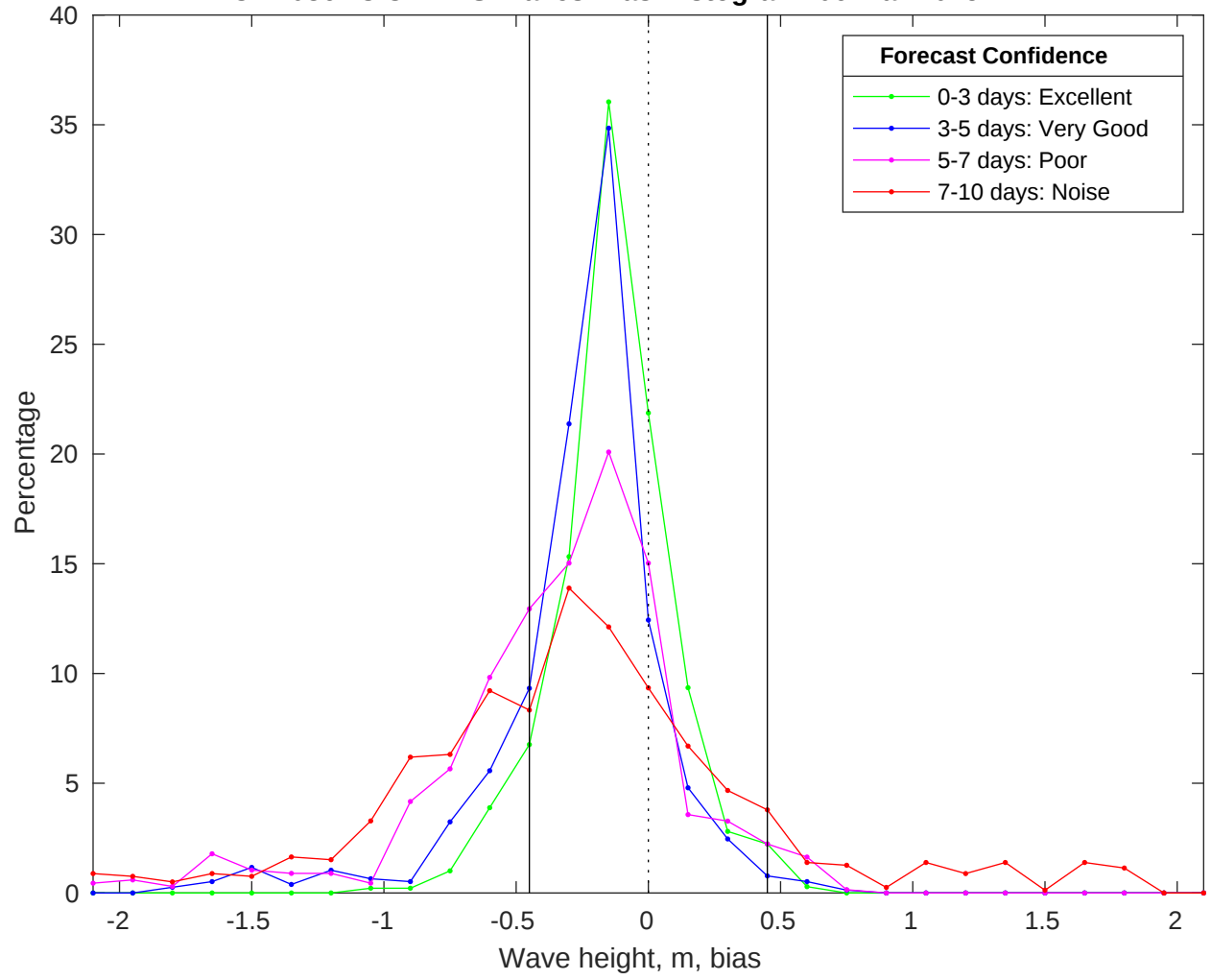
NDBC 42036 vs CMEMS Waves Bias Histogram: 06-Mar-2025
