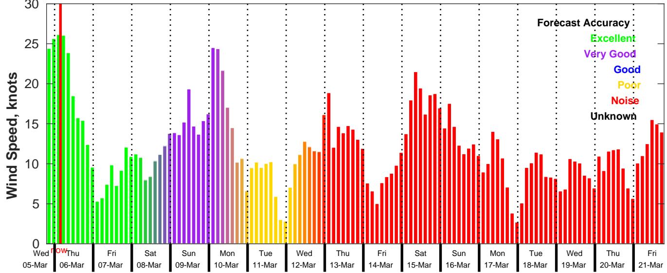
GFS Wind Speed Forecast for NDBC 42036 from 05-Mar-2025 19:00:00 to 21-Mar-2025 19:00:00
