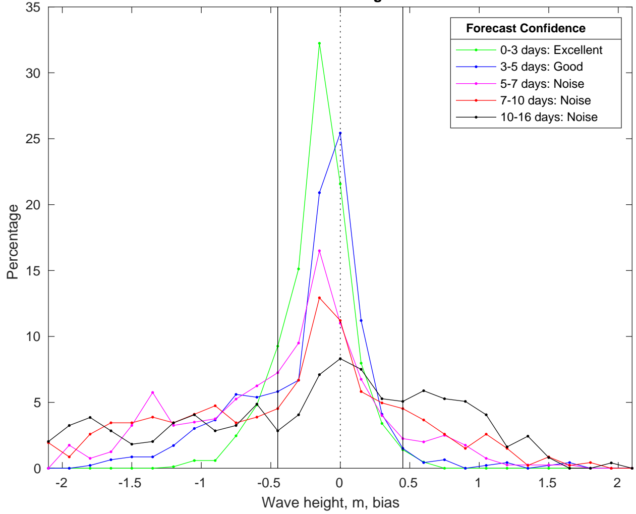
NDBC 42040 vs GFS Waves Bias Histogram: 06-Mar-2025
