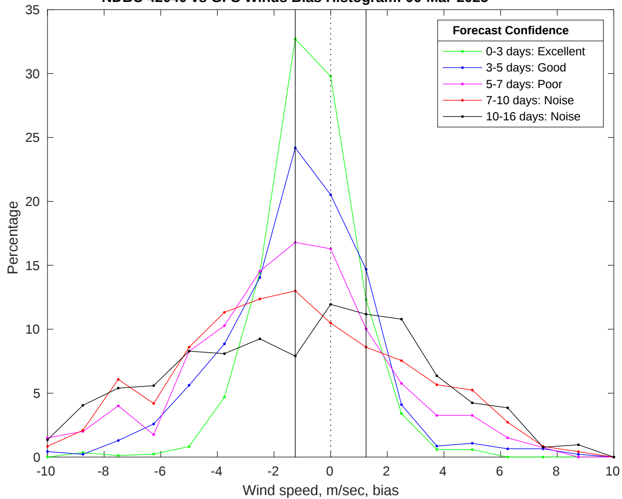
NDBC 42040 vs GFS Winds Bias Histogram: 06-Mar-2025
