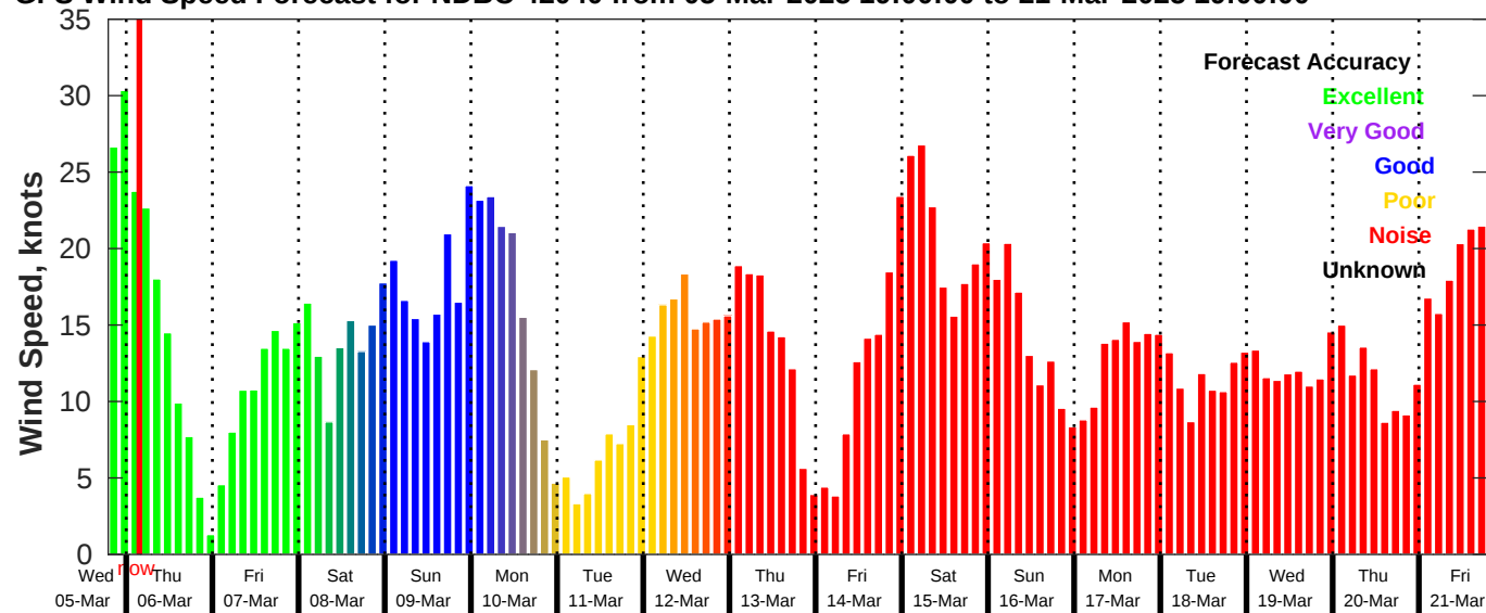
GFS Wind Speed Forecast for NDBC 42040 from 05-Mar-2025 19:00:00 to 21-Mar-2025 19:00:00
