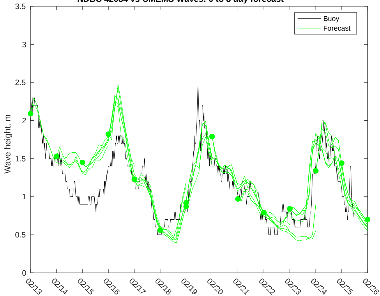
NDBC 42084 vs CMEMS Waves: 0 to 3 day forecast
