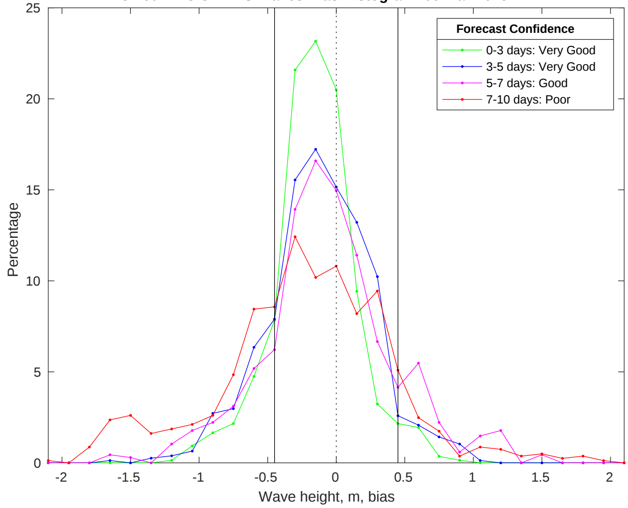
NDBC 46011 vs CMEMS Waves Bias Histogram: 06-Mar-2025
