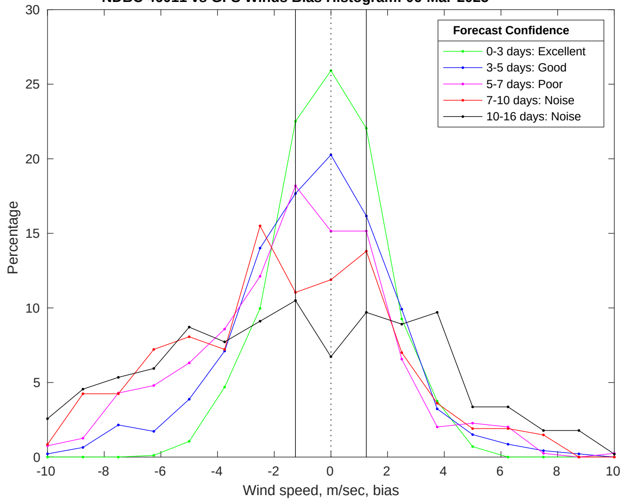
NDBC 46011 vs GFS Winds Bias Histogram: 06-Mar-2025
