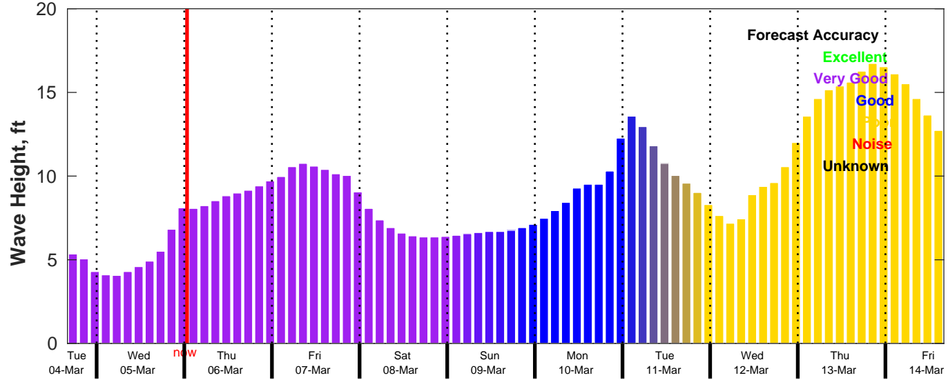
CMEMS Wave Forecast for NDBC 46011 from 04-Mar-2025 16:00:00 to 14-Mar-2025 16:00:00
