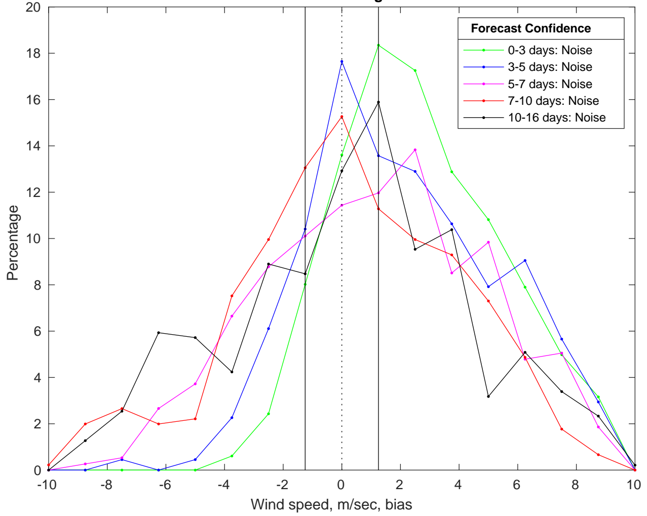
NDBC 46053 vs GFS Winds Bias Histogram: 05-Mar-2025
