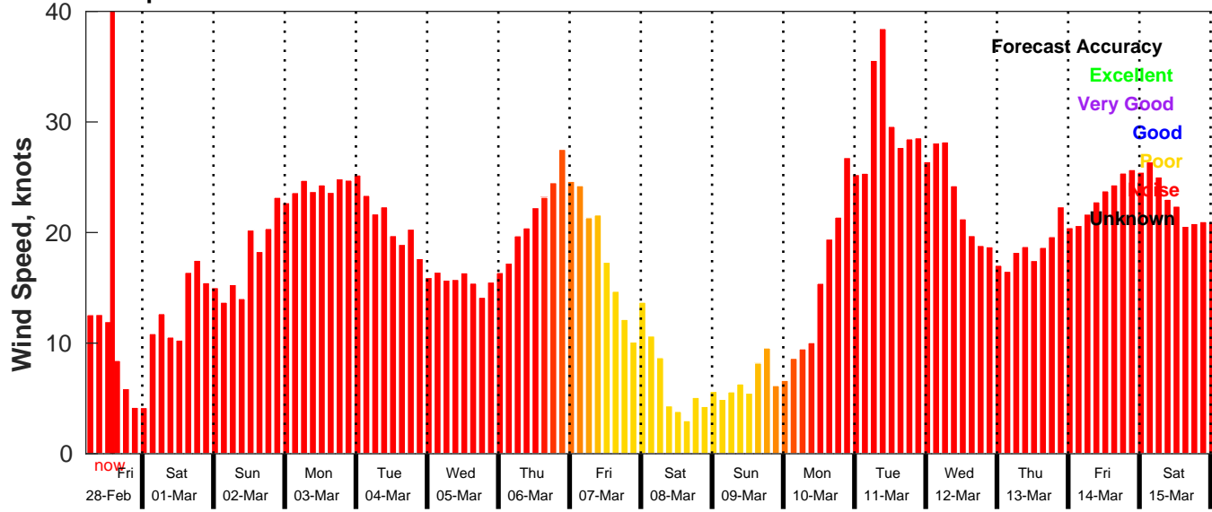
GFS Wind Speed Forecast for NDBC 46053 from 28-Feb-2025 05:00:00 to 16-Mar-2025 05:00:00
