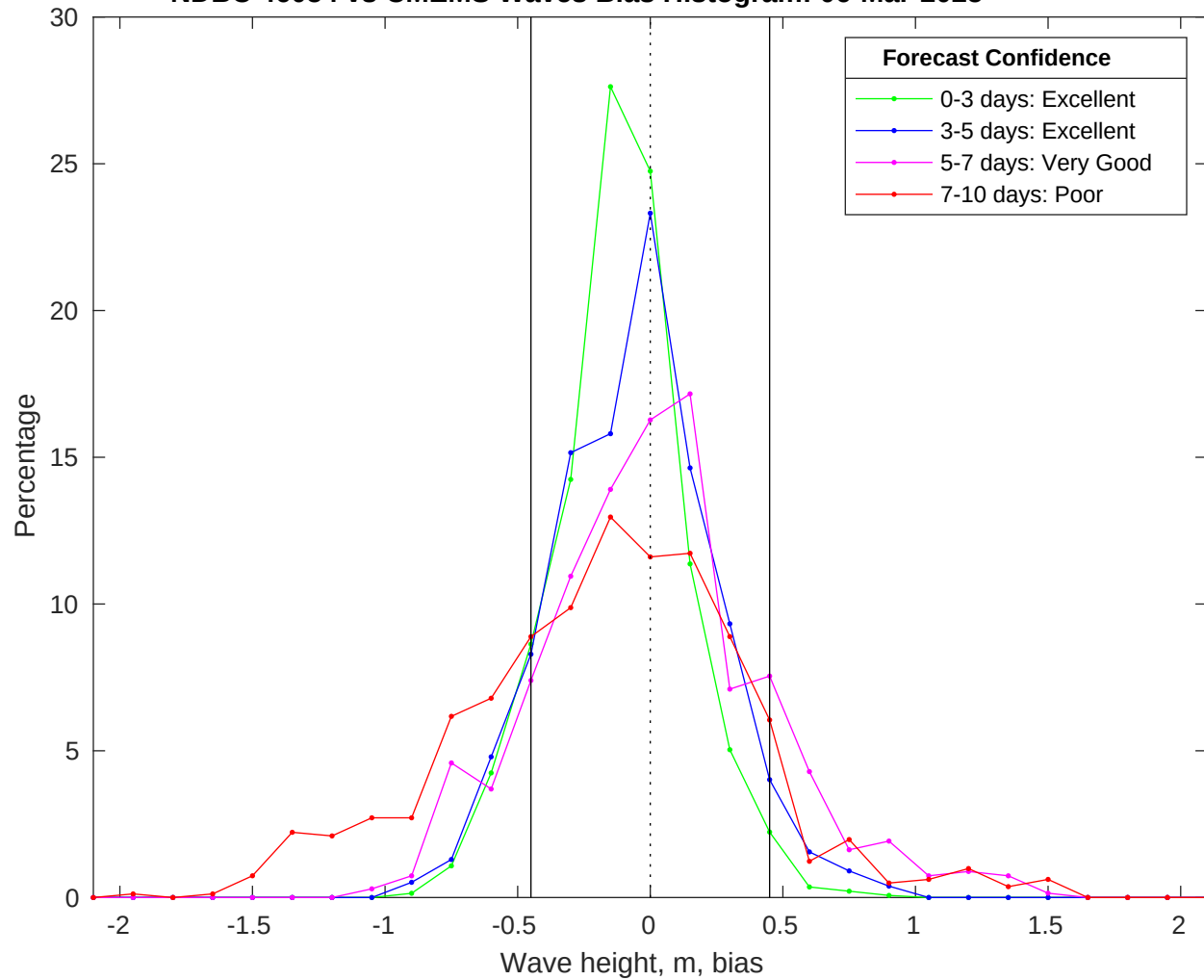
NDBC 46054 vs CMEMS Waves Bias Histogram: 06-Mar-2025
