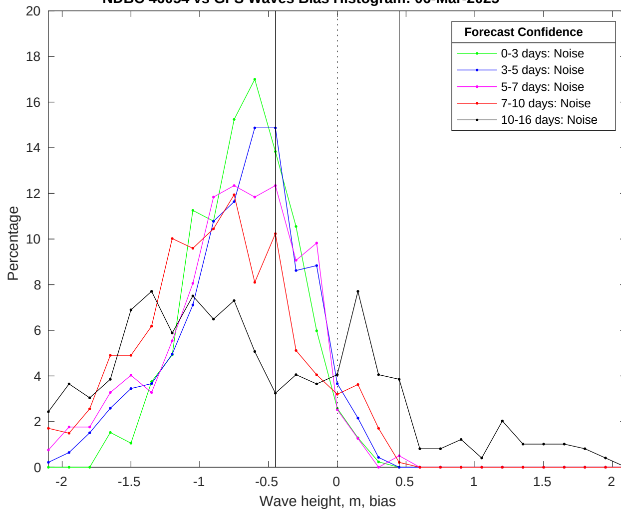
NDBC 46054 vs GFS Waves Bias Histogram: 06-Mar-2025
