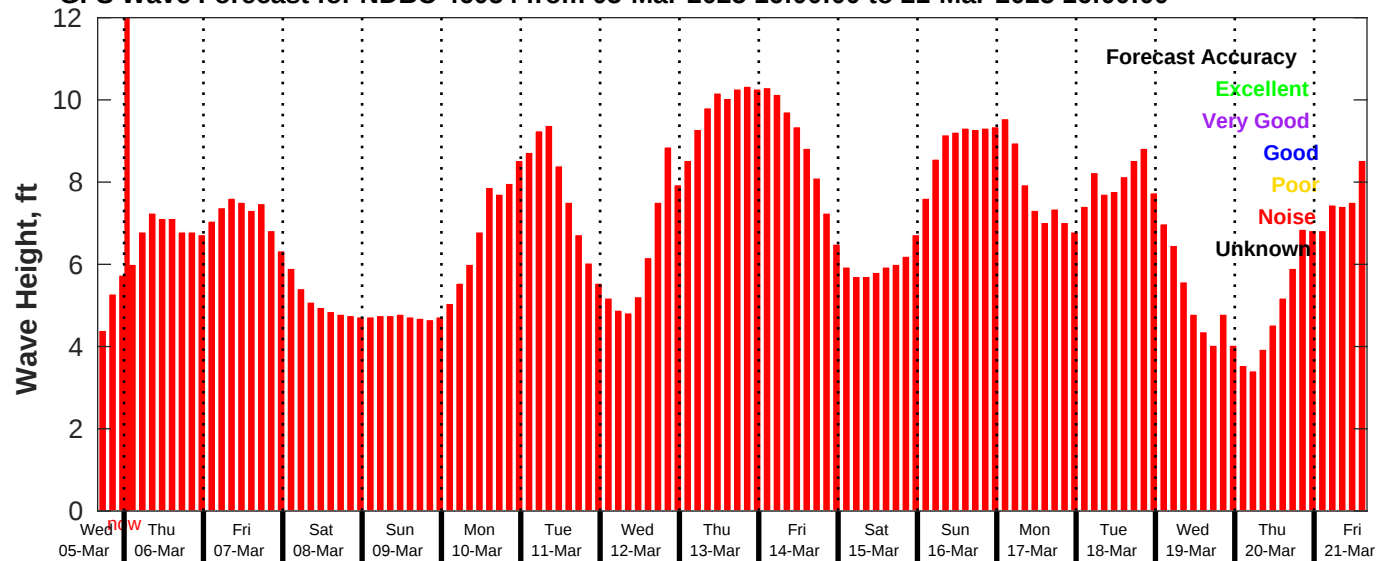
GFS Wave Forecast for NDBC 46054 from 05-Mar-2025 16:00:00 to 21-Mar-2025 16:00:00
