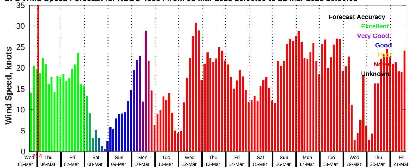
GFS Wind Speed Forecast for NDBC 46054 from 05-Mar-2025 16:00:00 to 21-Mar-2025 16:00:00
