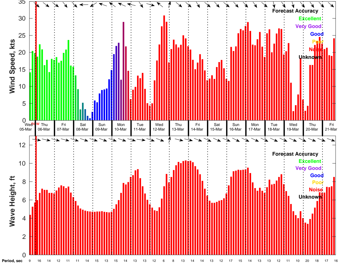
Wind & Wave Forecast for NDBC 46054 from 05-Mar-2025 16:00:00 to 21-Mar-2025 16:00:00
