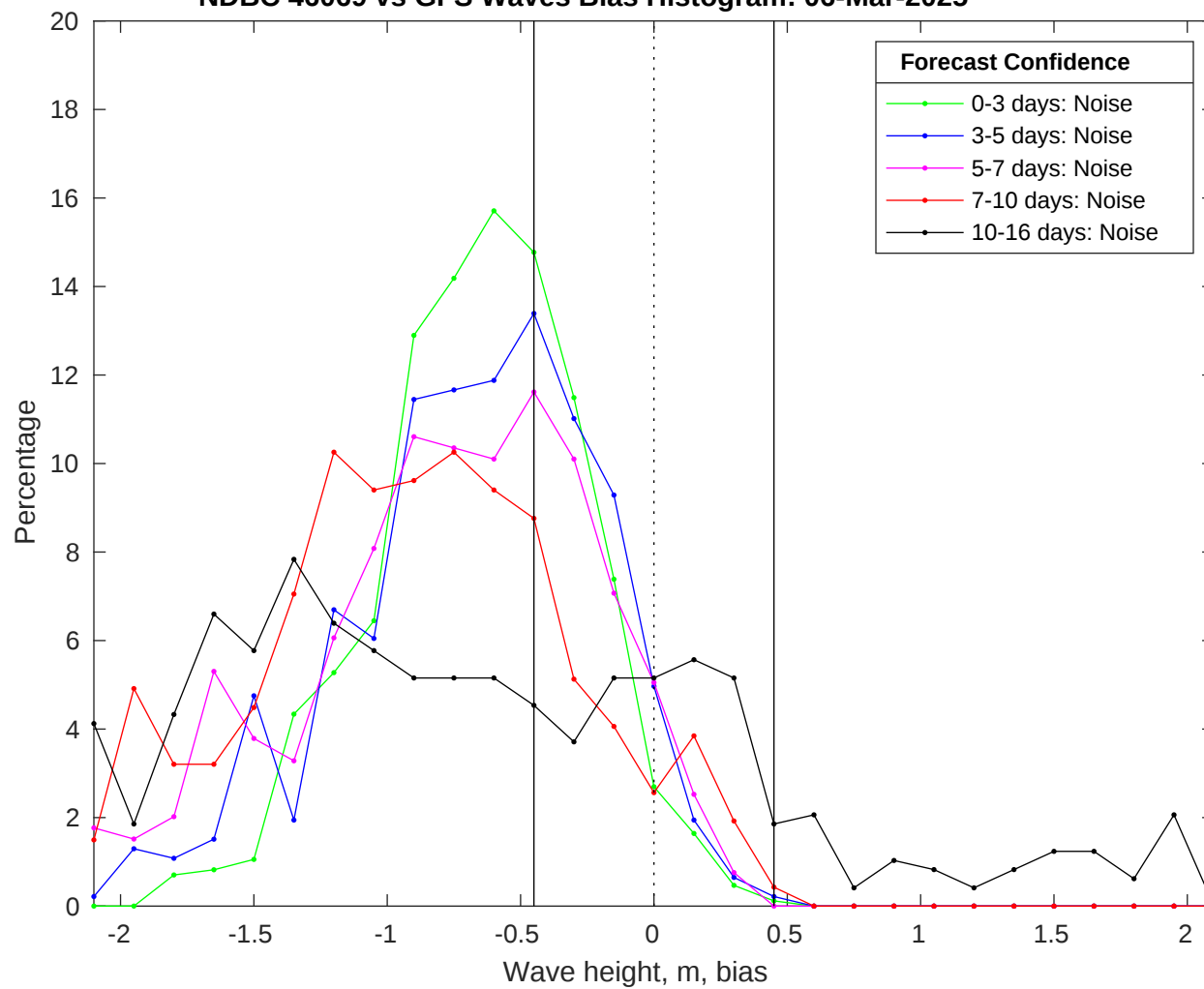
NDBC 46069 vs GFS Waves Bias Histogram: 06-Mar-2025
