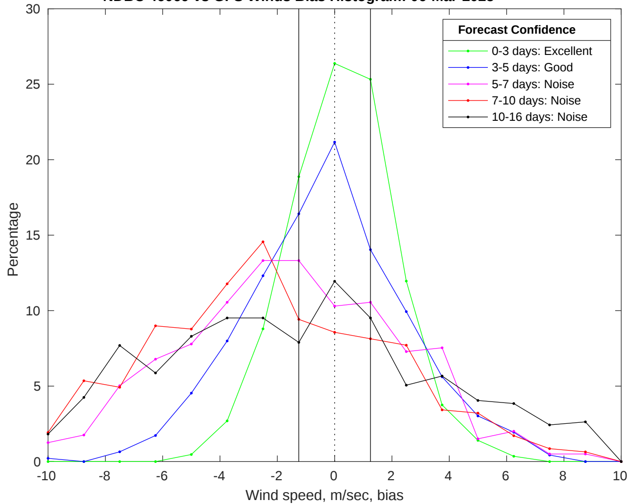
NDBC 46069 vs GFS Winds Bias Histogram: 06-Mar-2025
