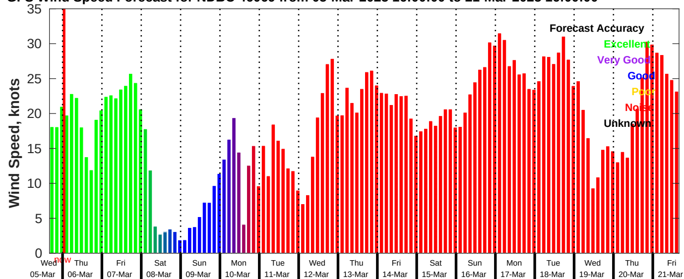
GFS Wind Speed Forecast for NDBC 46069 from 05-Mar-2025 16:00:00 to 21-Mar-2025 16:00:00
