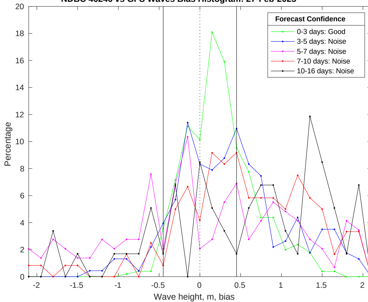
NDBC 46246 vs GFS Waves Bias Histogram: 27-Feb-2025
