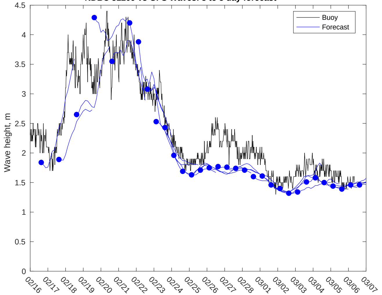
NDBC 51209 vs GFS Waves: 3 to 5 day forecast
