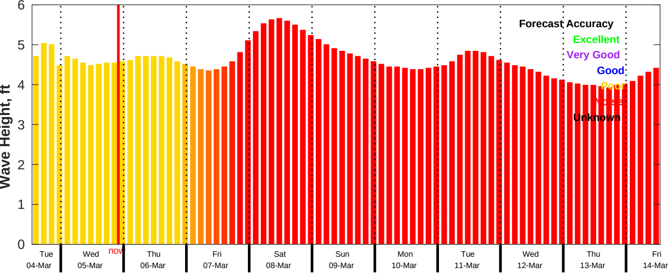
CMEMS Wave Forecast for NDBC 51209 from 04-Mar-2025 13:00:00 to 14-Mar-2025 13:00:00
