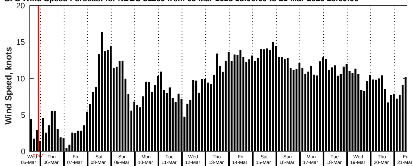
GFS Wind Speed Forecast for NDBC 51209 from 05-Mar-2025 13:00:00 to 21-Mar-2025 13:00:00
