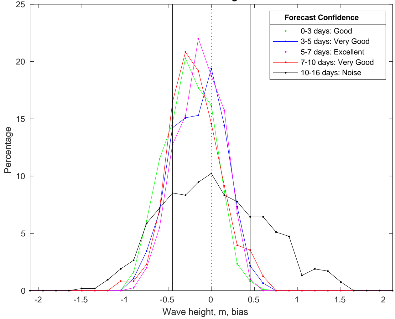
NDBC 52211 vs GFS Waves Bias Histogram: 06-Mar-2025
