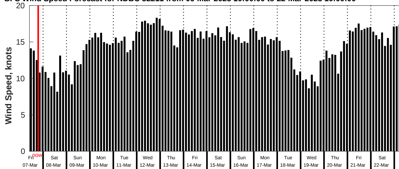
GFS Wind Speed Forecast for NDBC 52211 from 06-Mar-2025 10:00:00 to 22-Mar-2025 10:00:00
