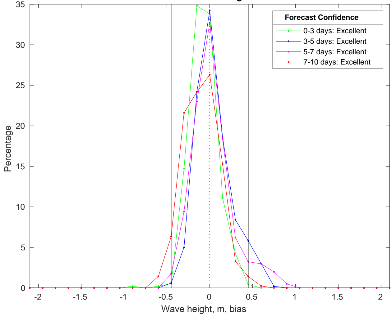
NDBC 52212 vs CMEMS Waves Bias Histogram: 06-Mar-2025
