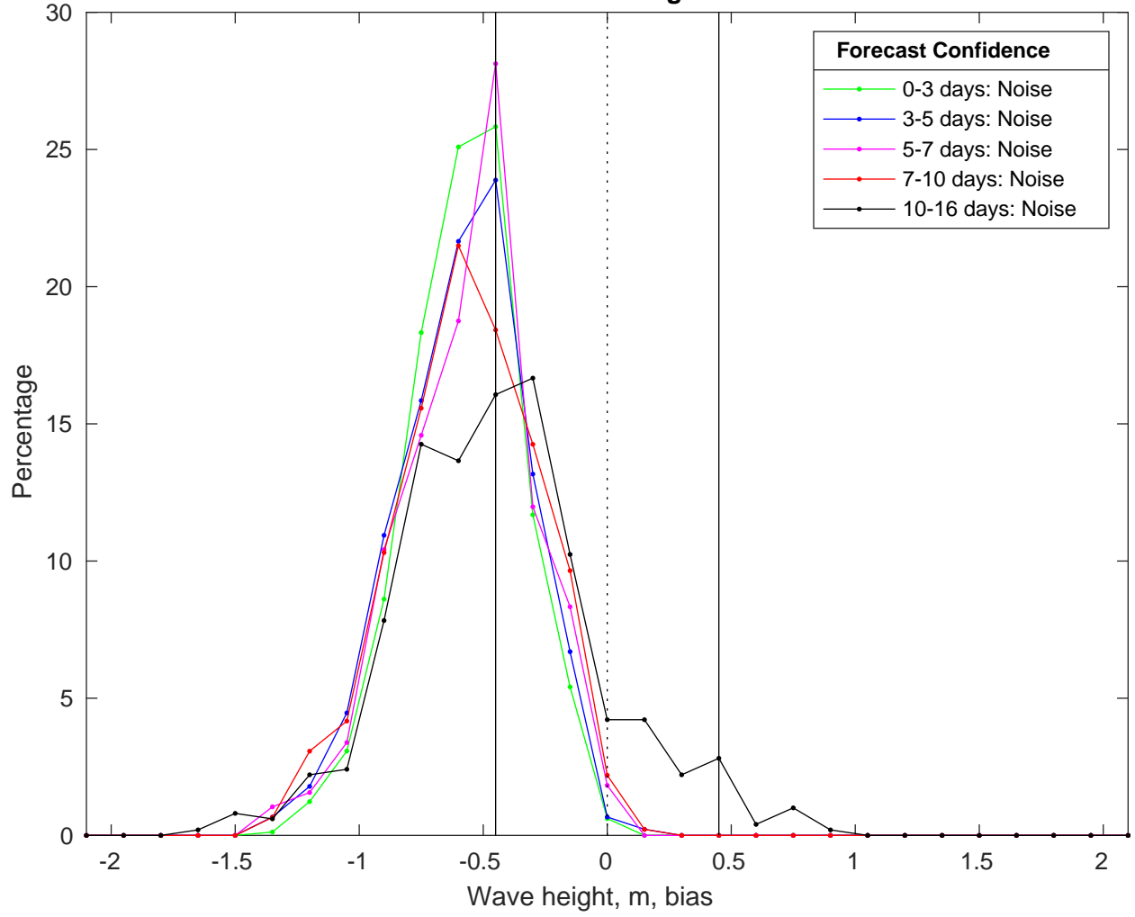
NDBC 52213 vs GFS Waves Bias Histogram: 06-Mar-2025
