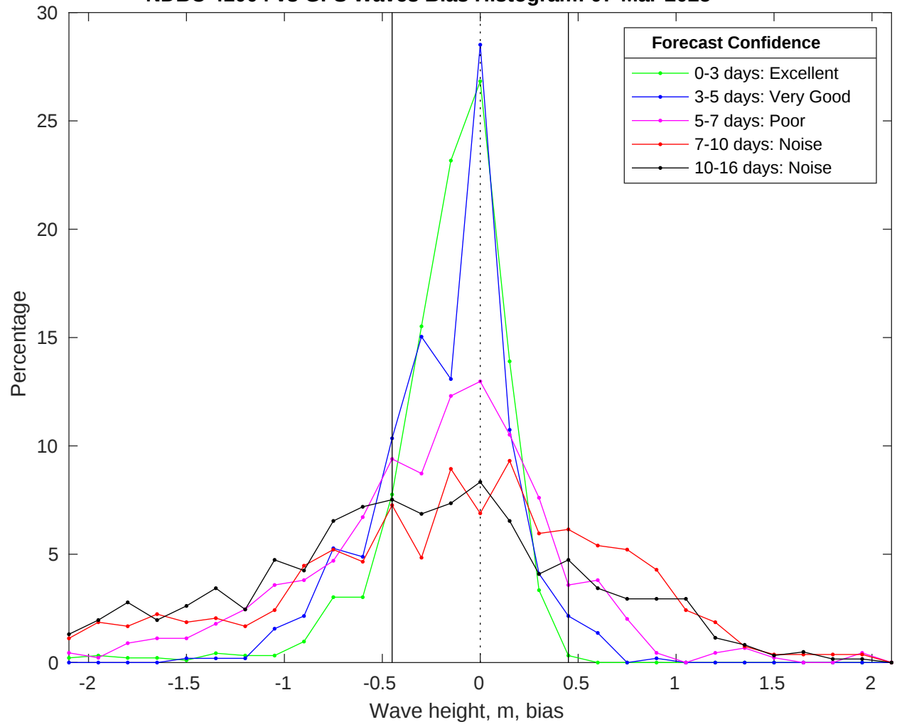
NDBC 41004 vs GFS Waves Bias Histogram: 07-Mar-2025
