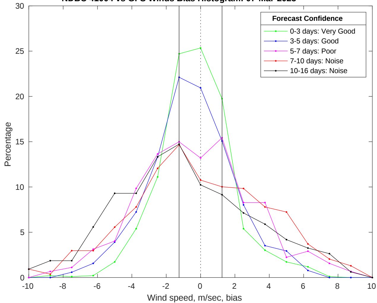
NDBC 41004 vs GFS Winds Bias Histogram: 07-Mar-2025
