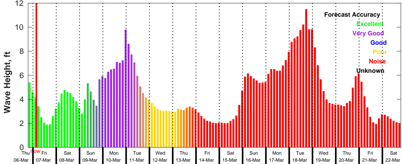
GFS Wave Forecast for NDBC 41004 from 06-Mar-2025 19:00:00 to 22-Mar-2025 19:00:00
