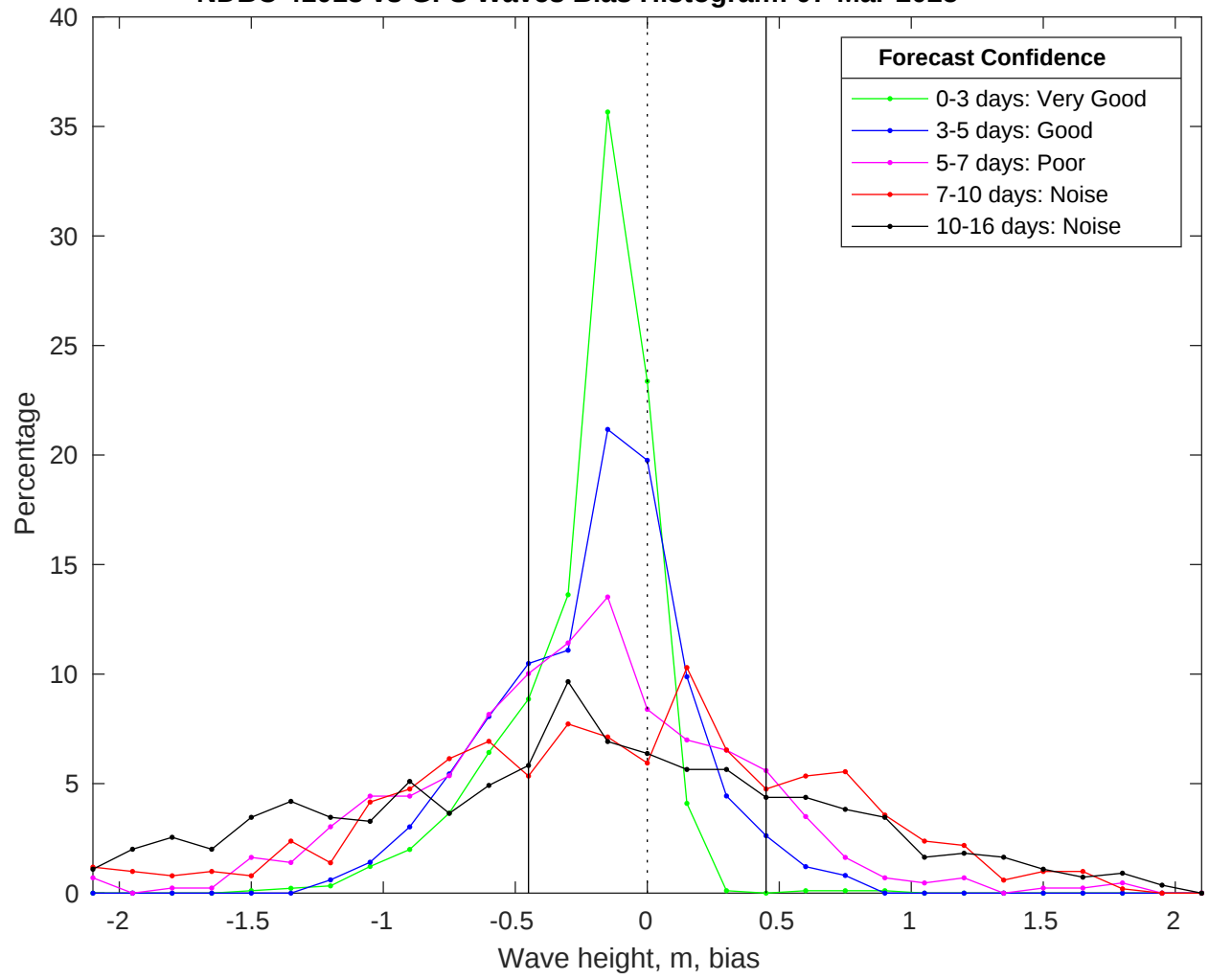
NDBC 41013 vs GFS Waves Bias Histogram: 07-Mar-2025
