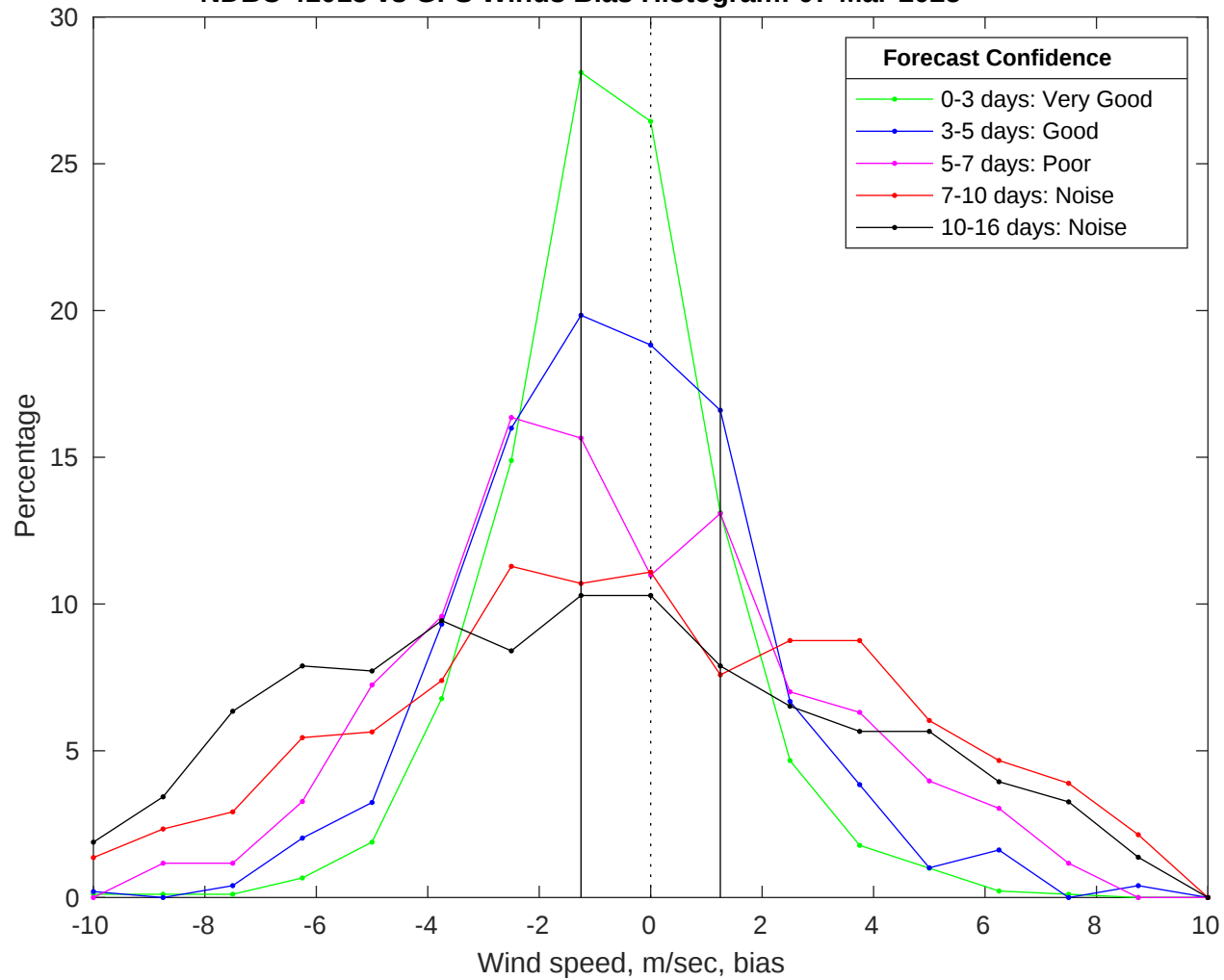
NDBC 41013 vs GFS Winds Bias Histogram: 07-Mar-2025
