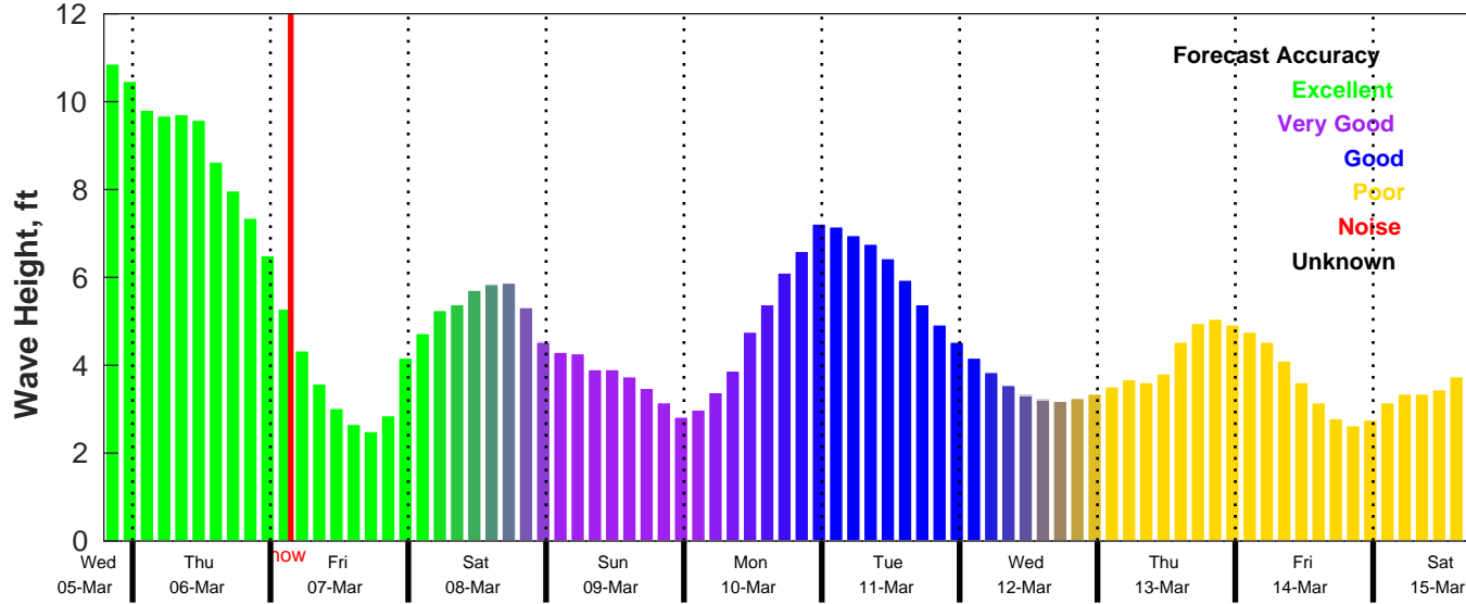
CMEMS Wave Forecast for NDBC 41013 from 05-Mar-2025 19:00:00 to 15-Mar-2025 19:00:00
