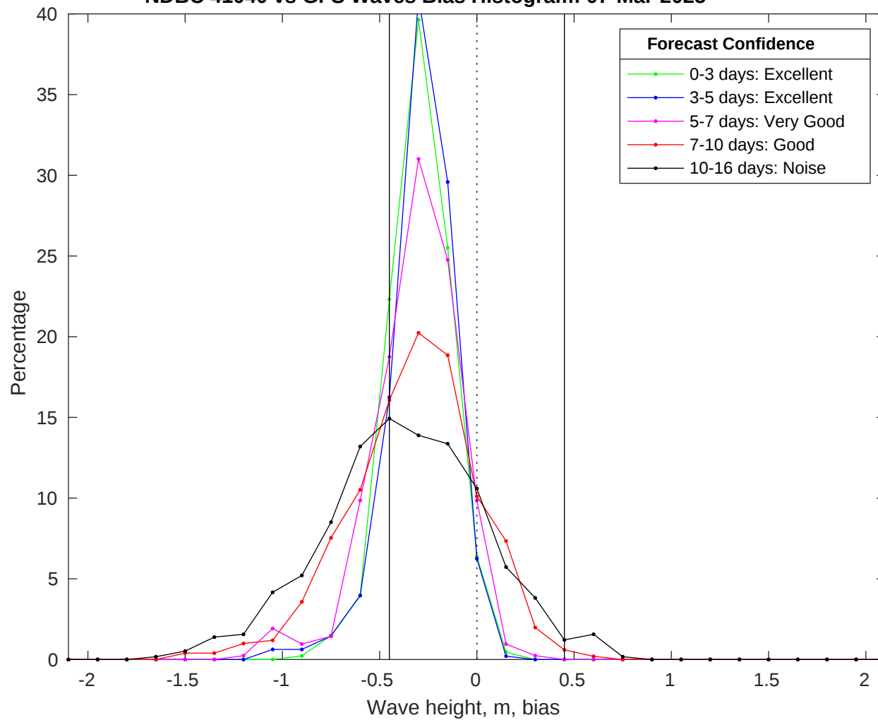
NDBC 41040 vs GFS Waves Bias Histogram: 07-Mar-2025
