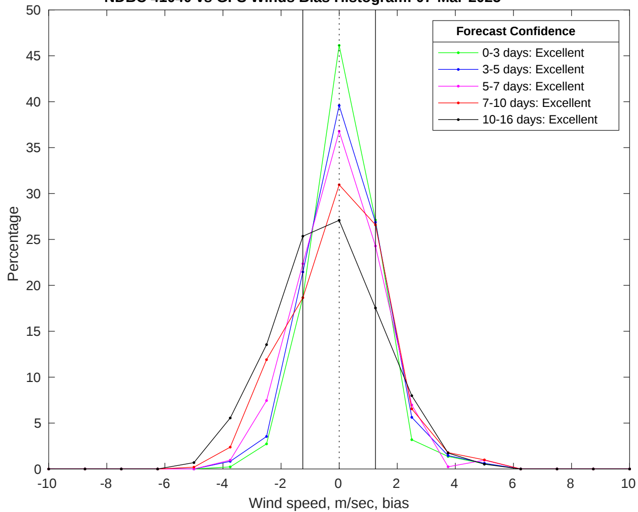
NDBC 41040 vs GFS Winds Bias Histogram: 07-Mar-2025
