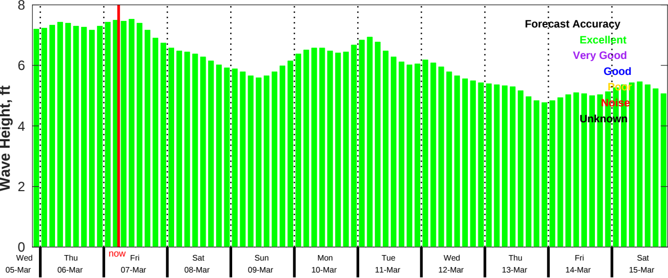
CMEMS Wave Forecast for NDBC 41040 from 05-Mar-2025 21:00:00 to 15-Mar-2025 21:00:00
