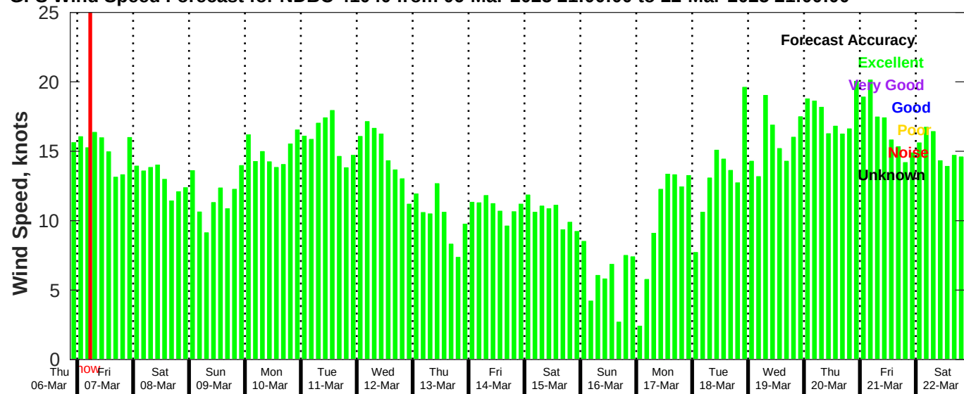
GFS Wind Speed Forecast for NDBC 41040 from 06-Mar-2025 21:00:00 to 22-Mar-2025 21:00:00
