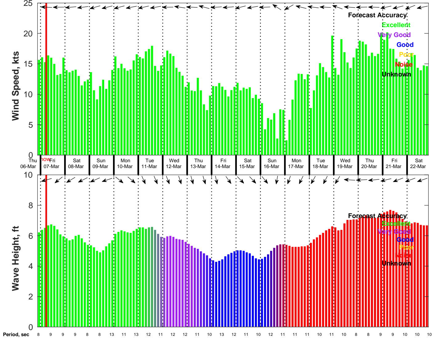
Wind & Wave Forecast for NDBC 41040 from 06-Mar-2025 21:00:00 to 22-Mar-2025 21:00:00
