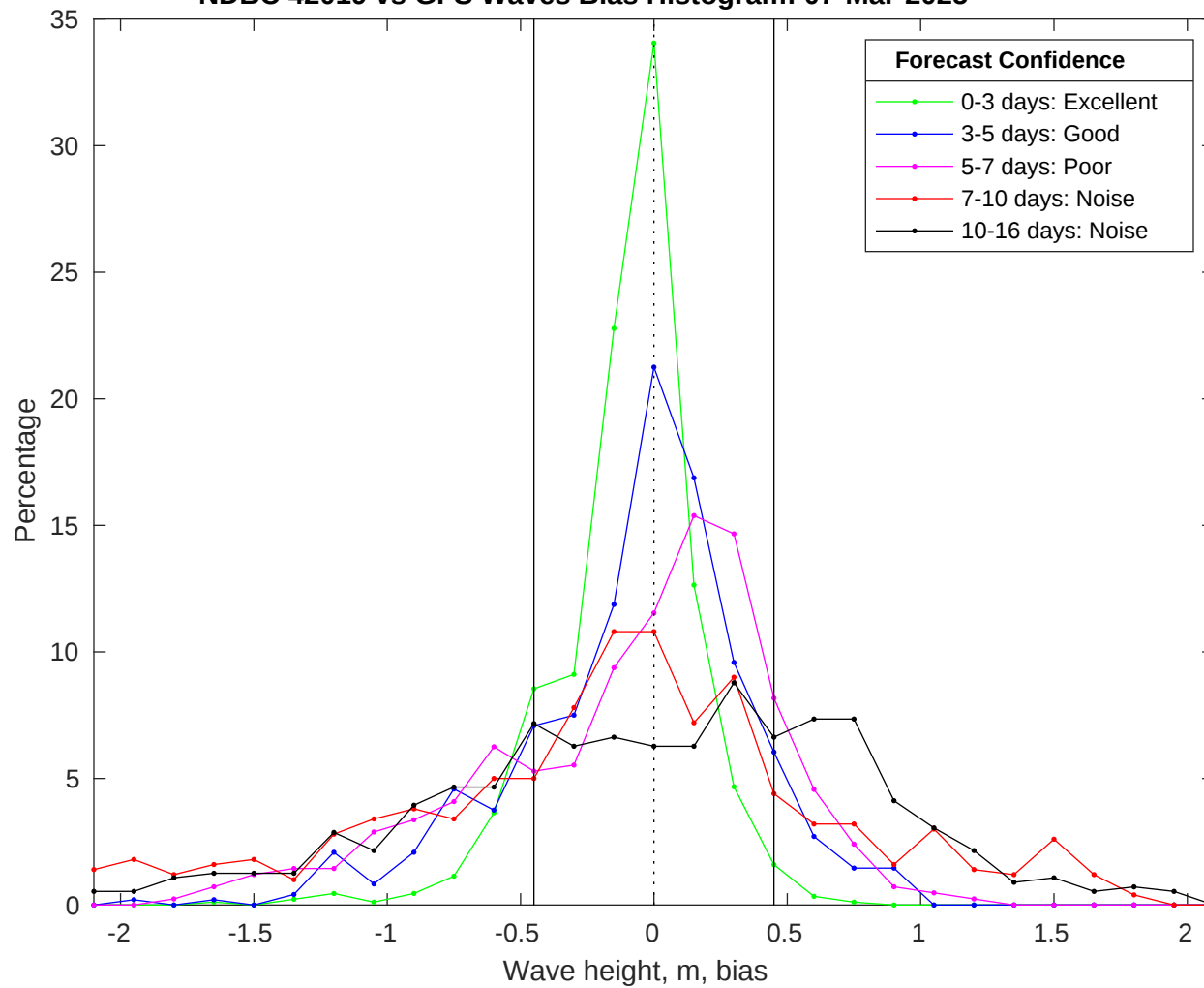
NDBC 42019 vs GFS Waves Bias Histogram: 07-Mar-2025
