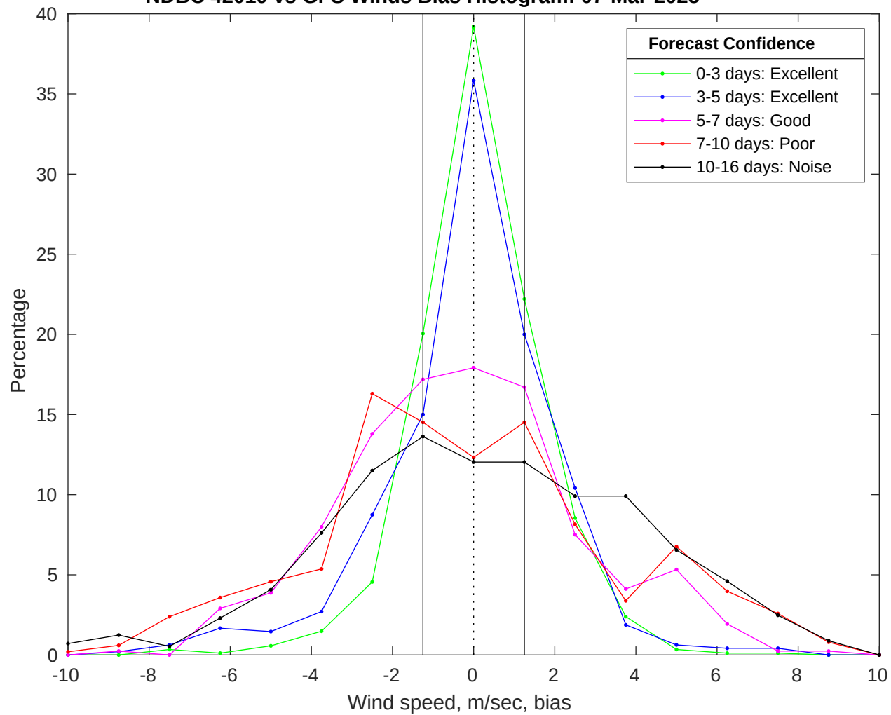
NDBC 42019 vs GFS Winds Bias Histogram: 07-Mar-2025
