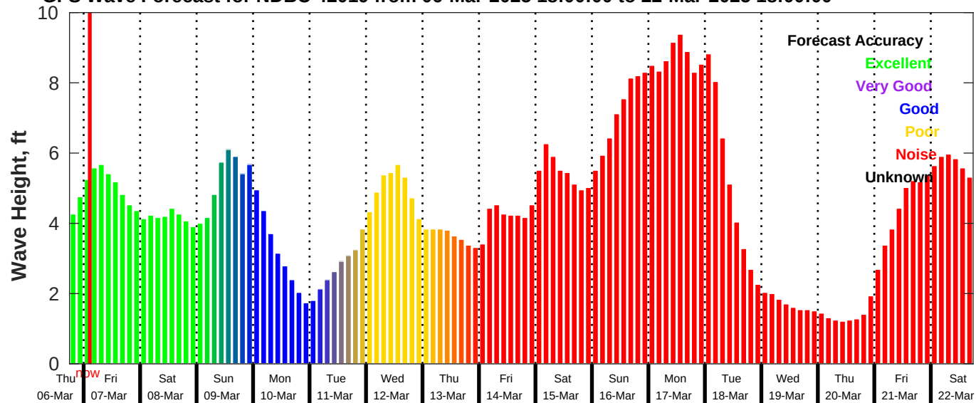
GFS Wave Forecast for NDBC 42019 from 06-Mar-2025 18:00:00 to 22-Mar-2025 18:00:00
